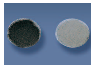
Carbon deposits in the filter paper three minutes after the cold start. With post-heating (on the right), carbon deposits are approx. 40% less than without post-heating.
